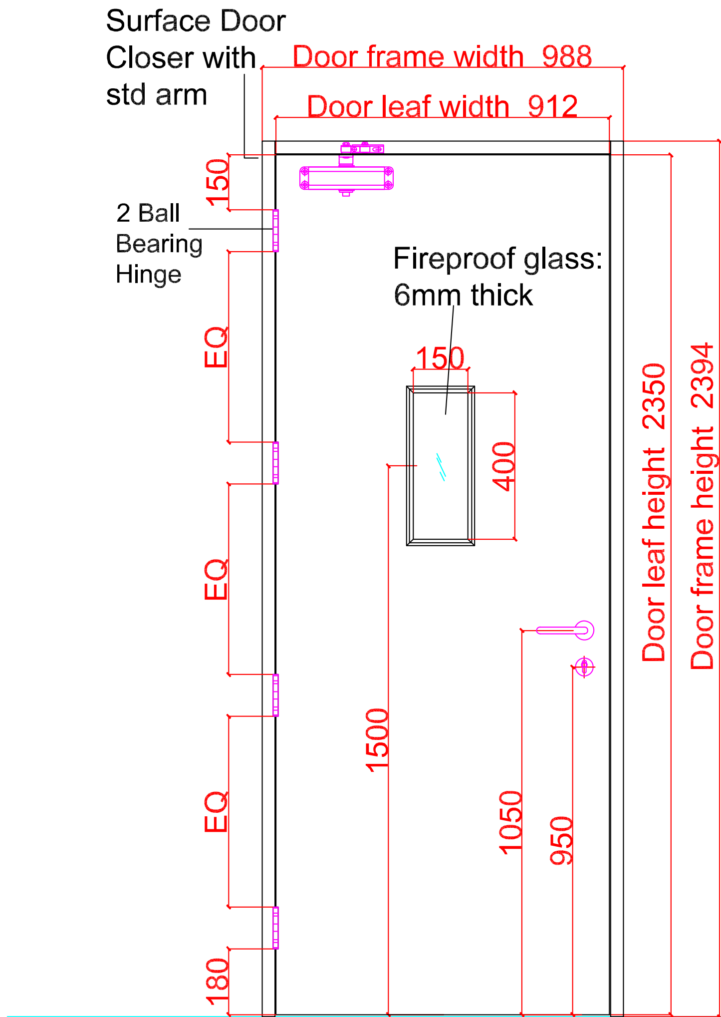
Outside elevation
