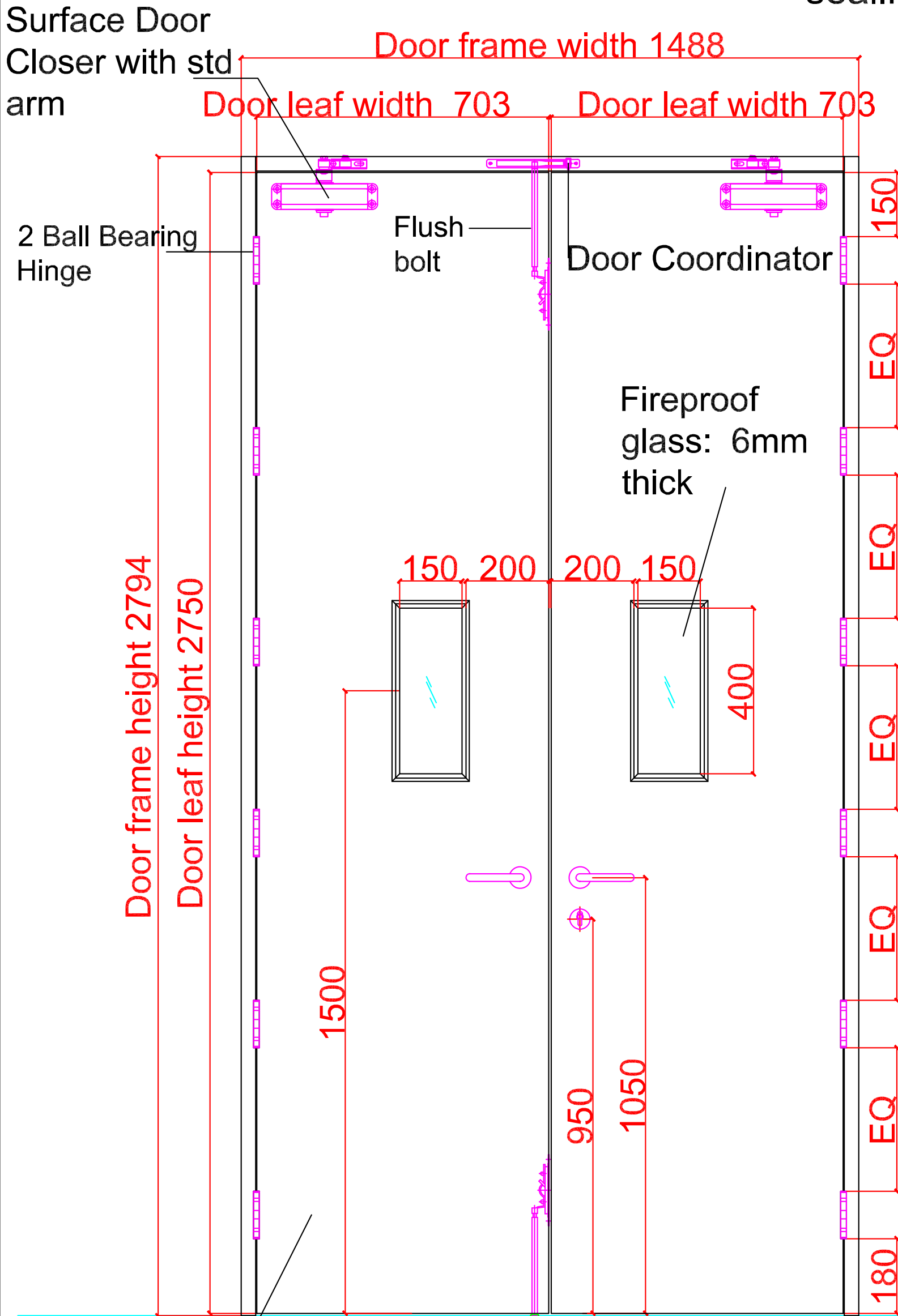
Outside elevation
