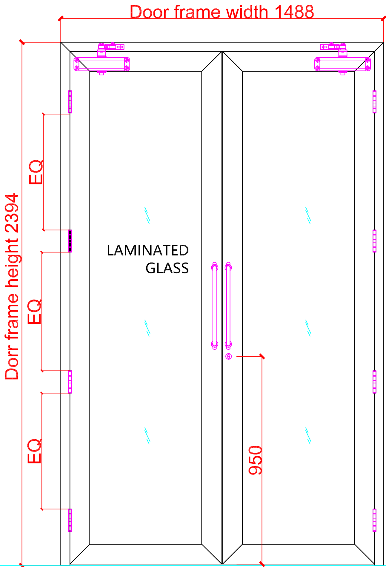
External elevation
