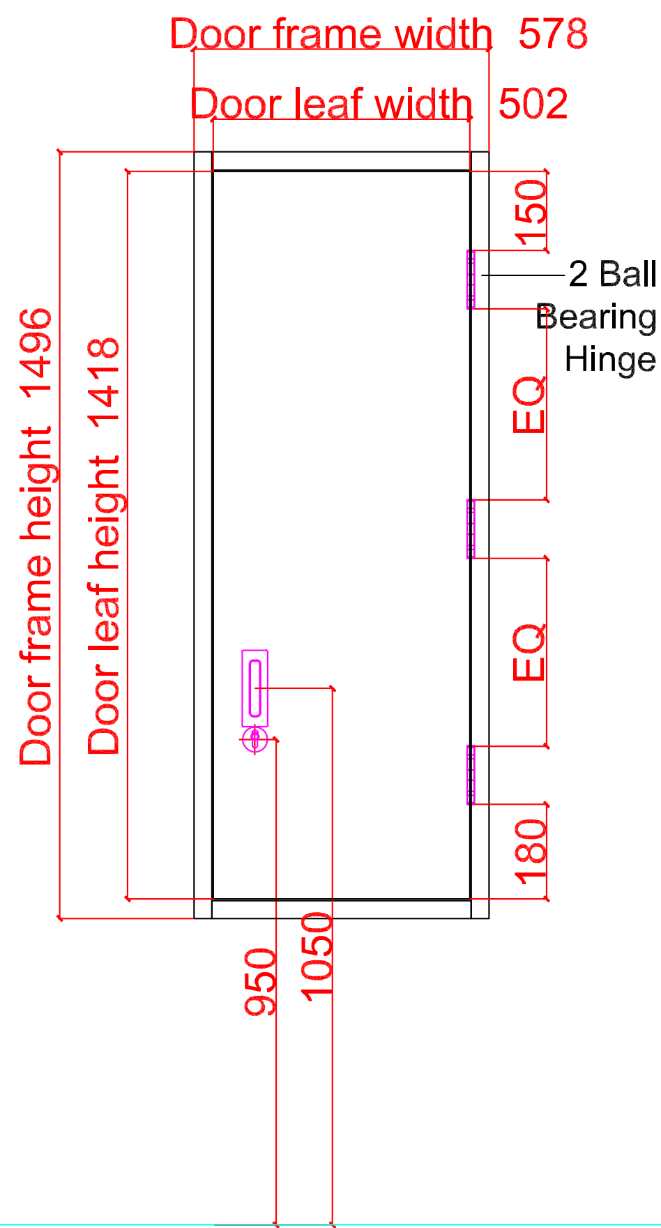
Outside elevation
