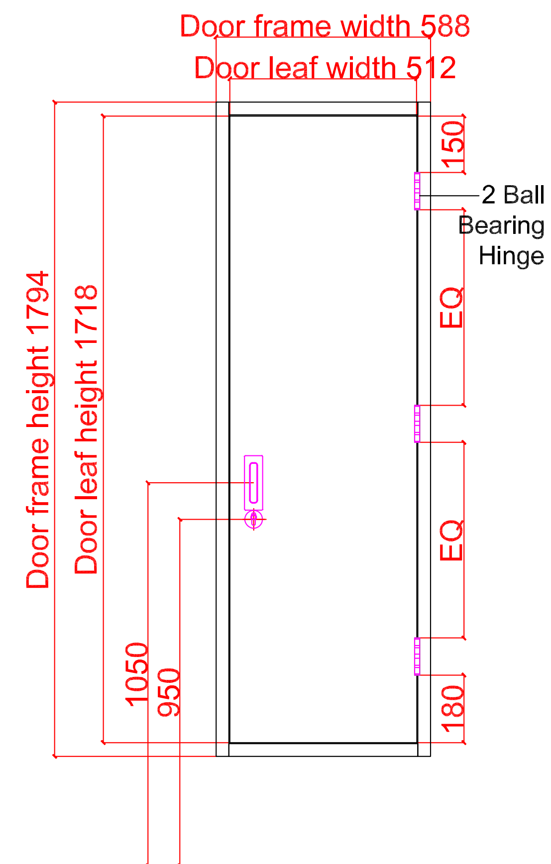
Outside elevation
