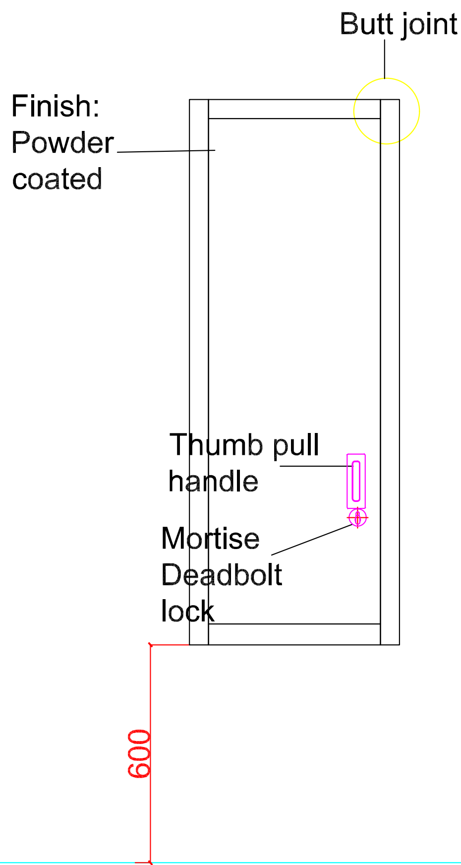
Inside elevation
