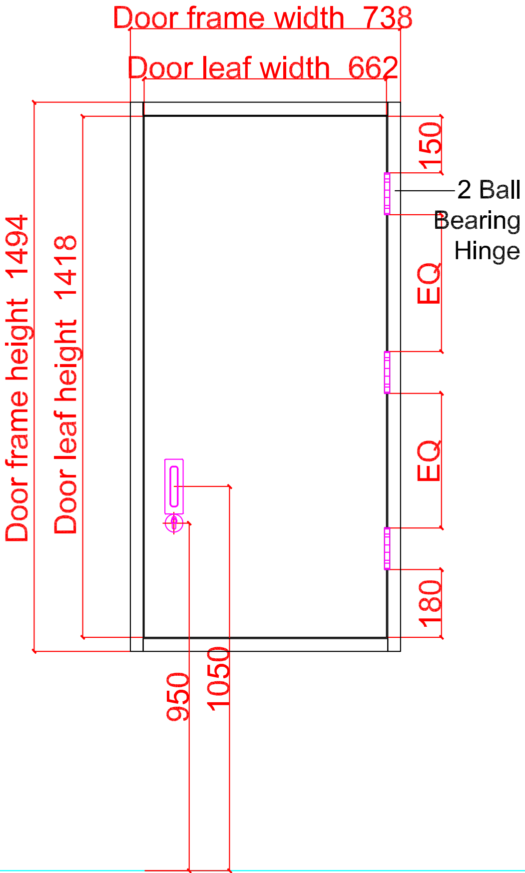
Outside elevation
