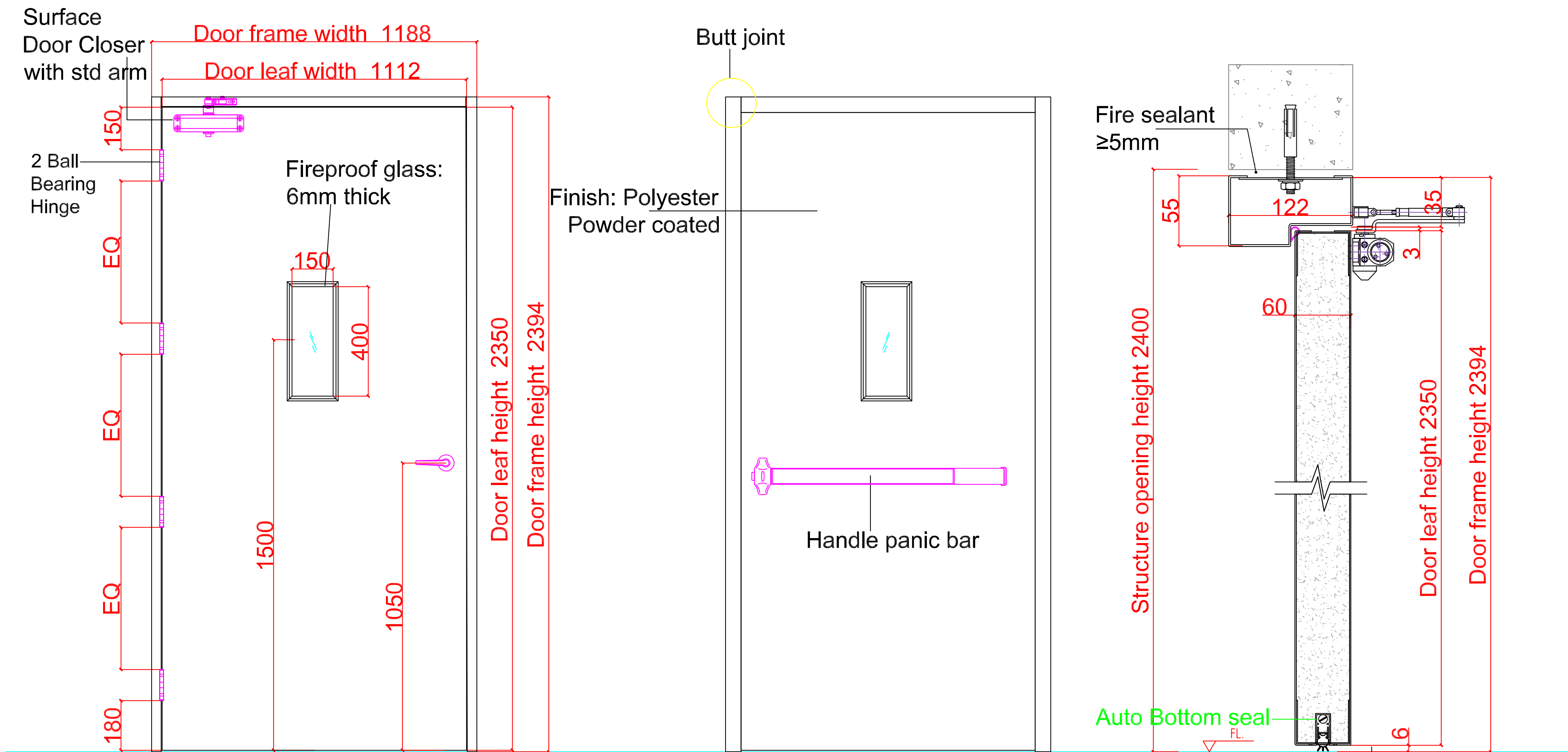
Outside elevation
