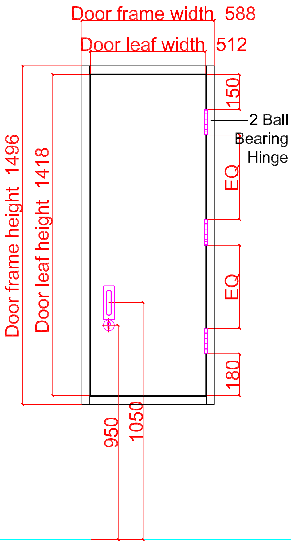
Outside elevation
