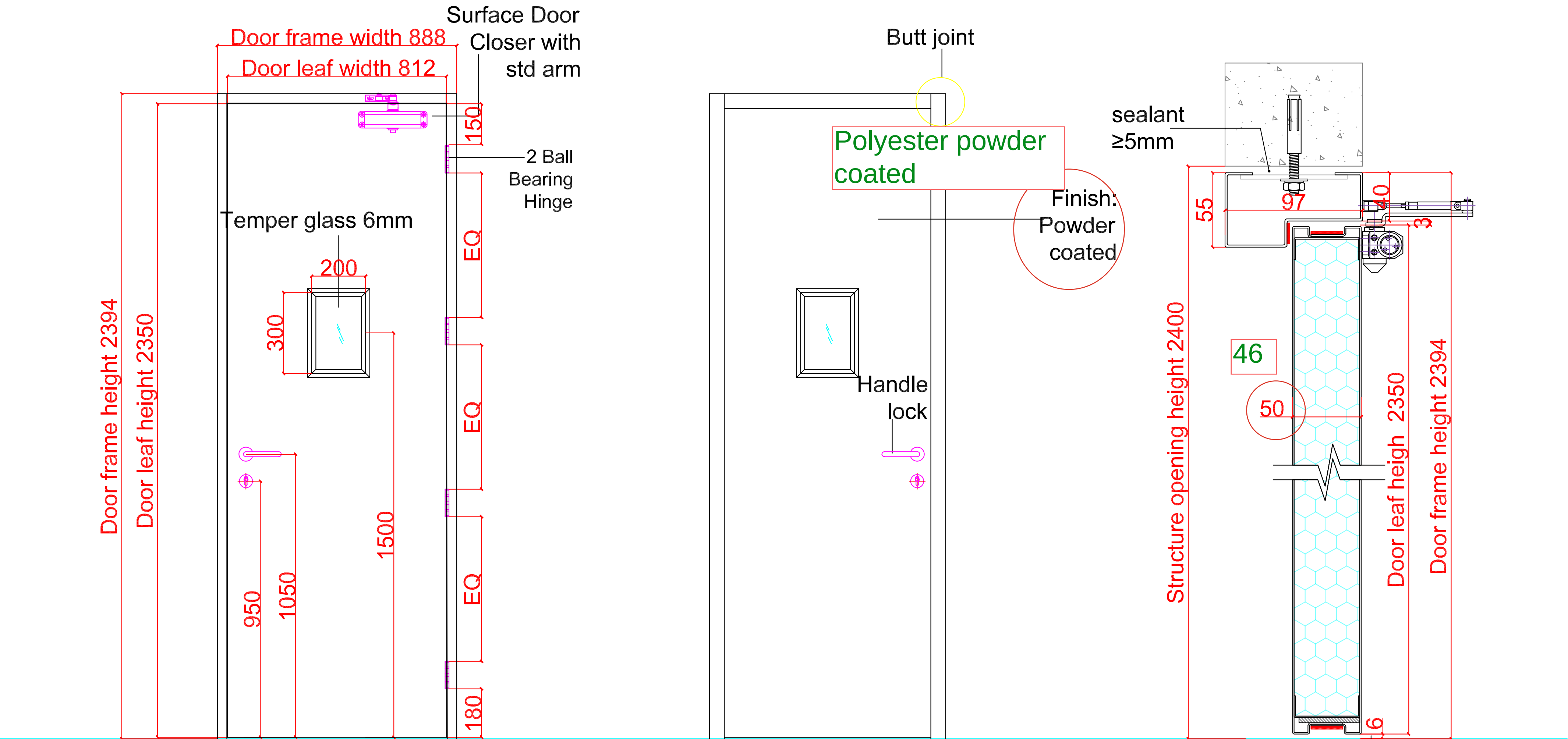
Outside elevation
