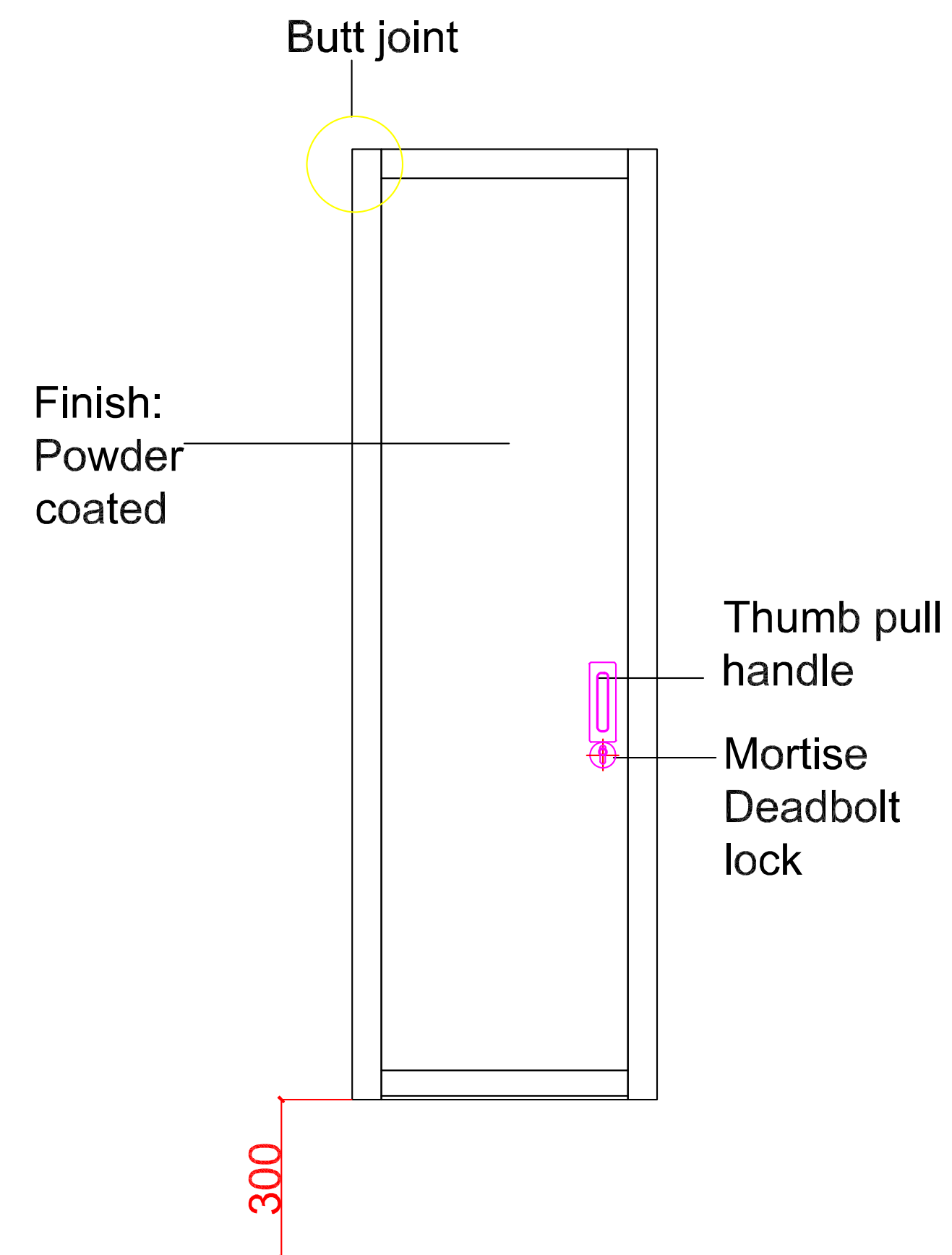
Inside elevation
