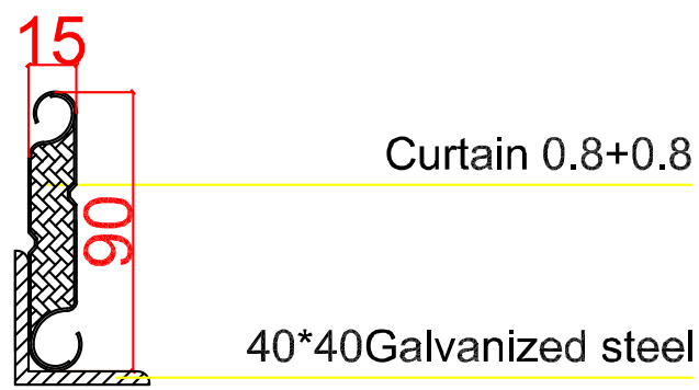
Bottom beam
