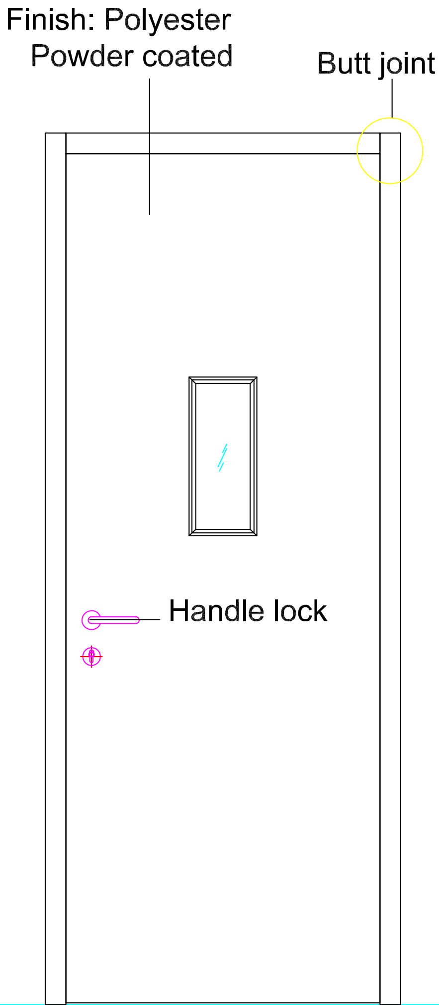
Inside elevation
