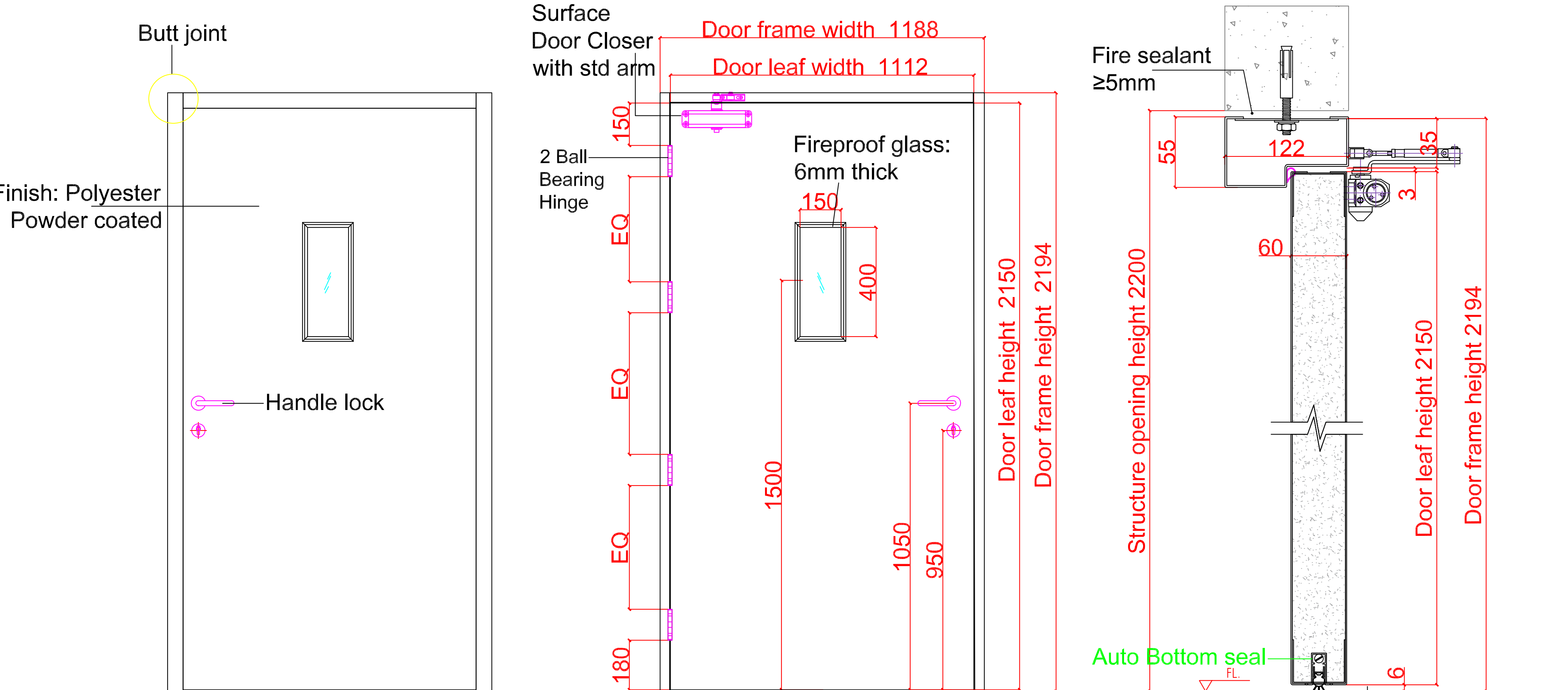
Outside elevation
