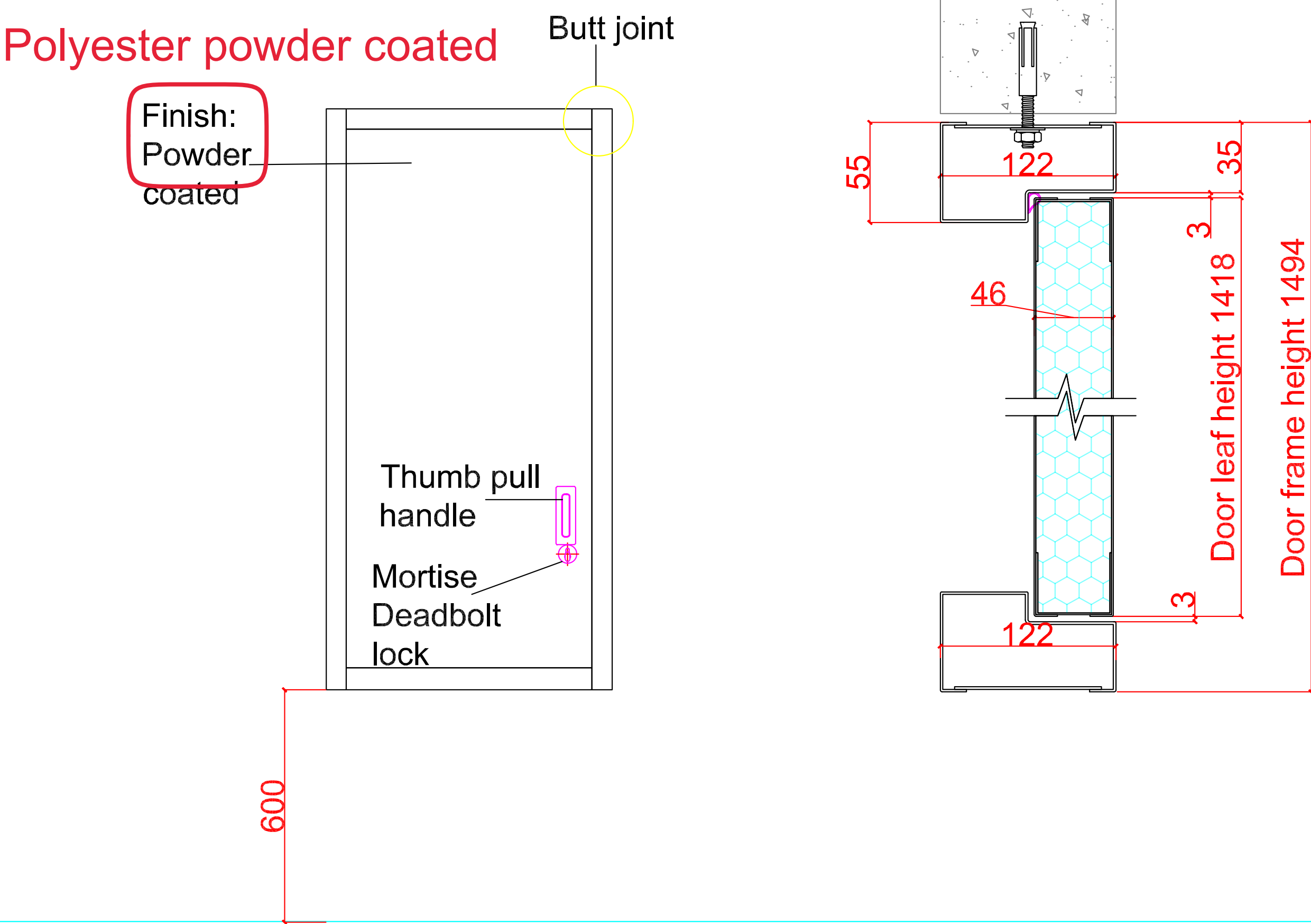
Inside elevation
