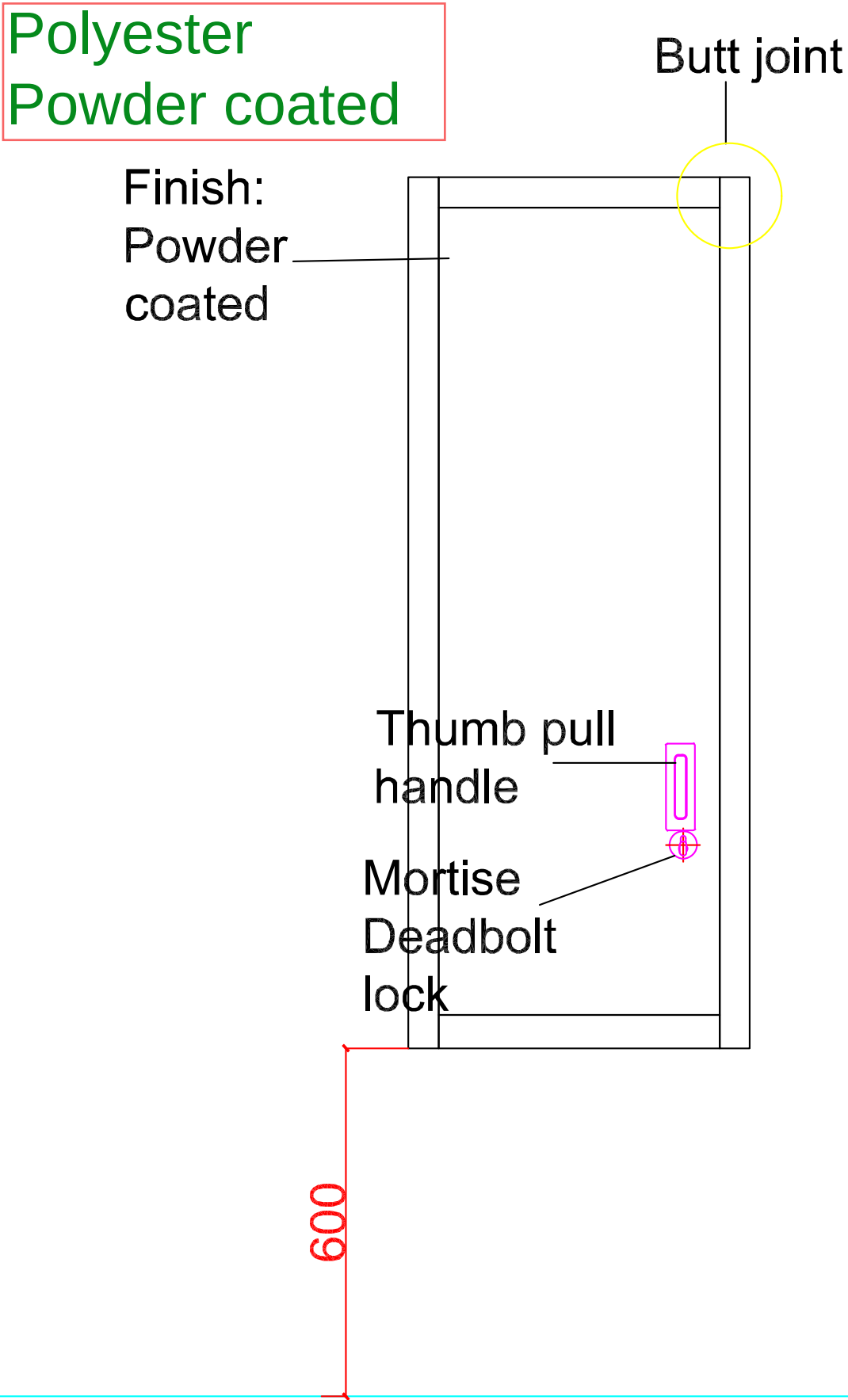
Inside elevation
