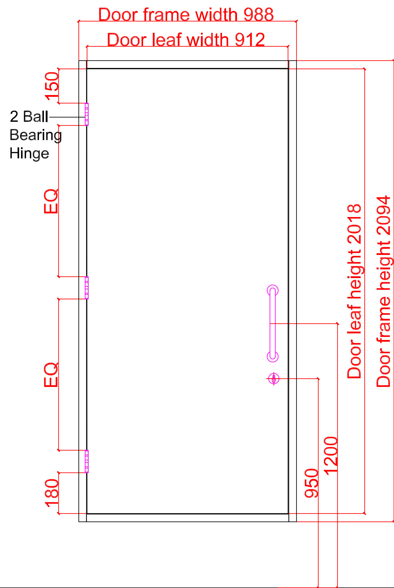
Outside elevation
